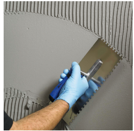
Using a suitable trowel, apply the second and possible third layer until the required total thickness is obtained.
